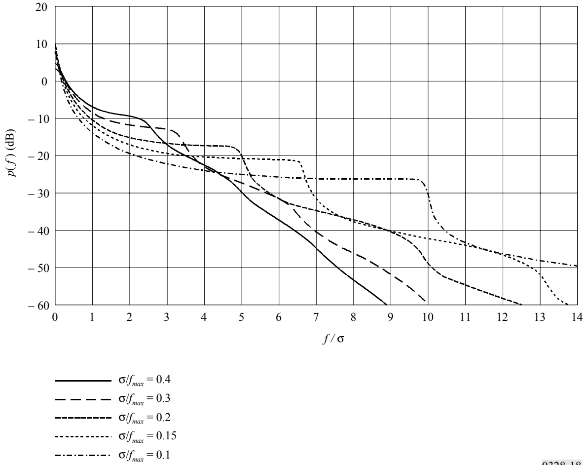
FIGURE 18 Power spectral distribution for \sigma/f_{max} < 0.5
