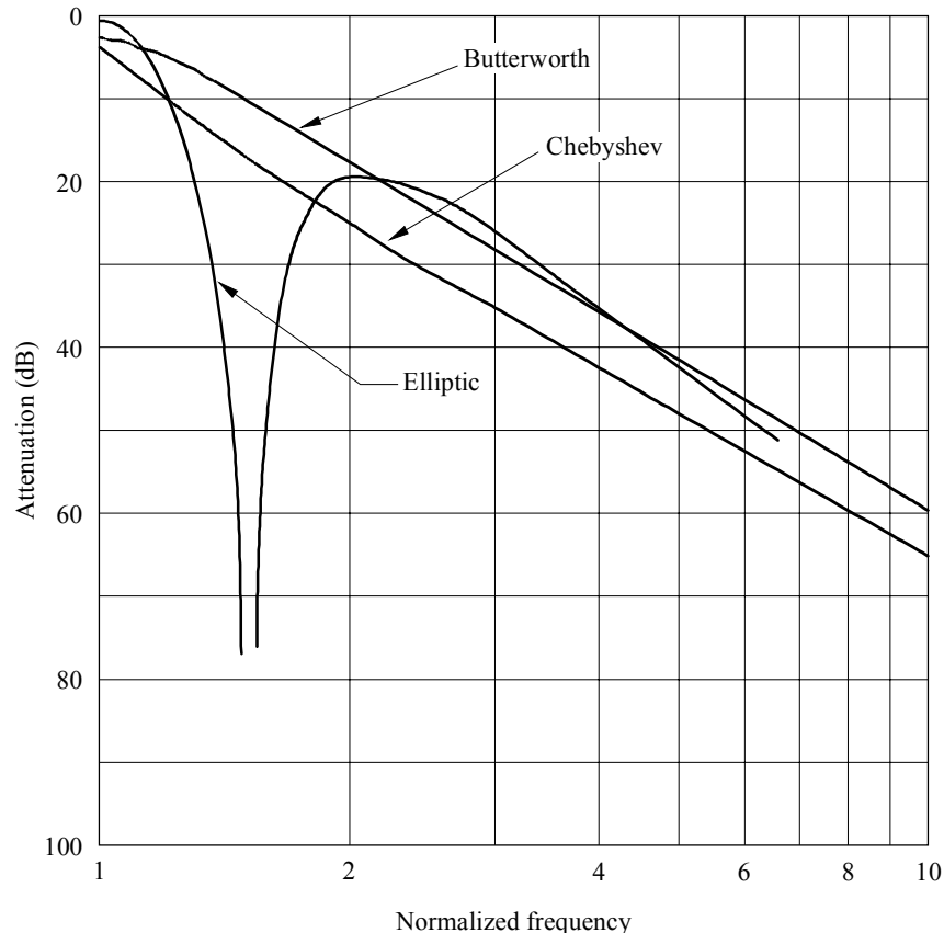
FIGURE 41 Comparison of Butterworth, Chebyshev and Elliptic filters, n = 3
