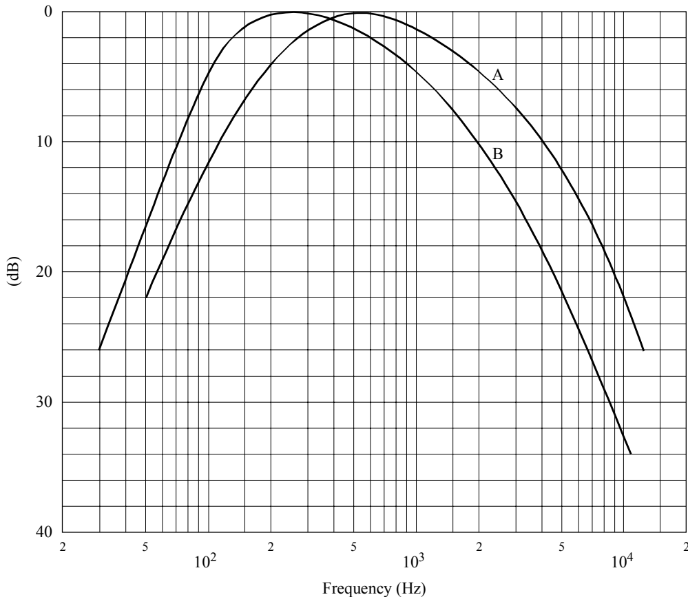
Curves A: frequency spectrum of standardized noise (measured with one-third octave filters) B: frequency response characteristic of filter-circuit
