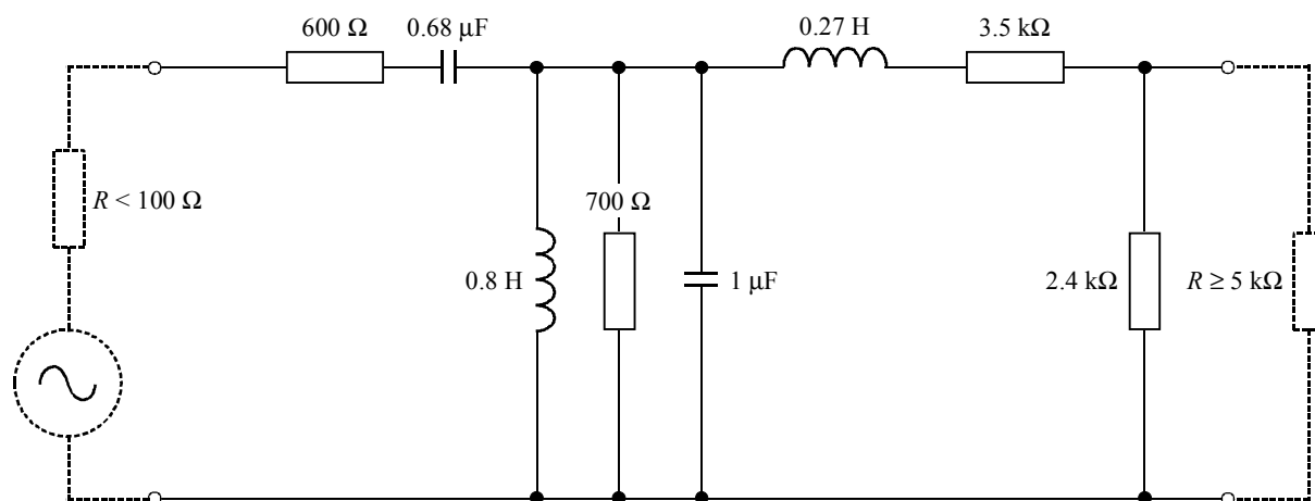
FIGURE 9 Filter circuit
