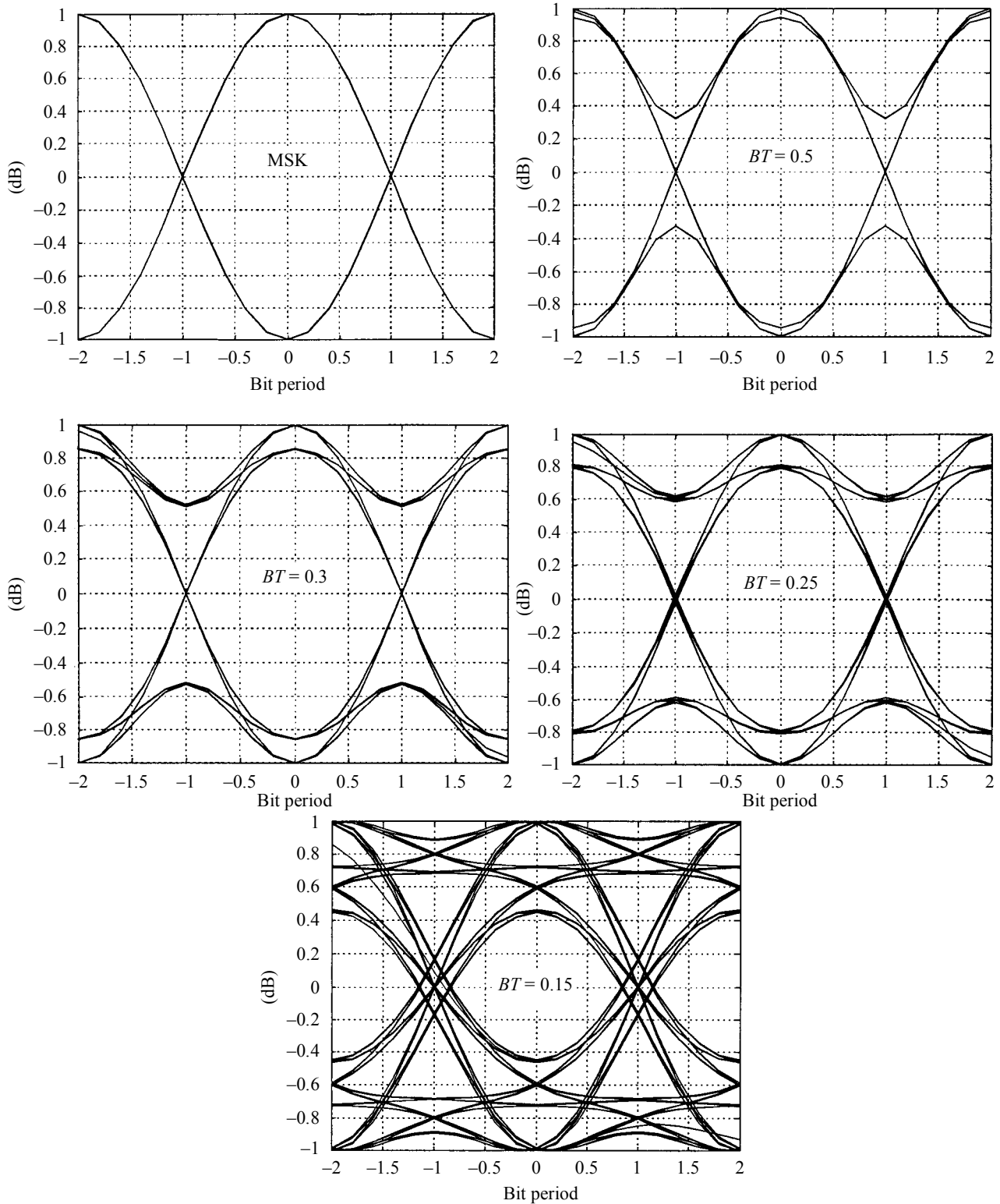
FIGURE 33 Eye diagrams
