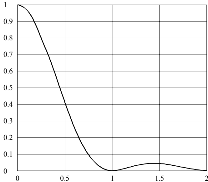
FIGURE 26 BPSK spectrum
