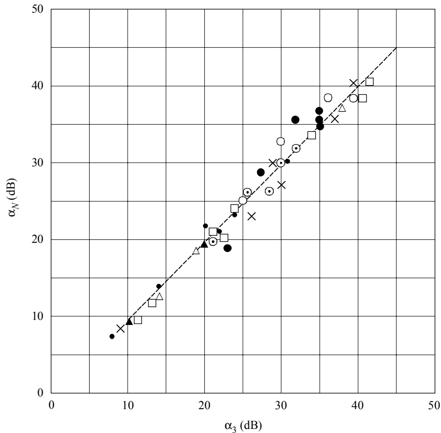
FIGURE 24 The value of \alpha_N shown in Fig. 23 for different values of \alpha_3
