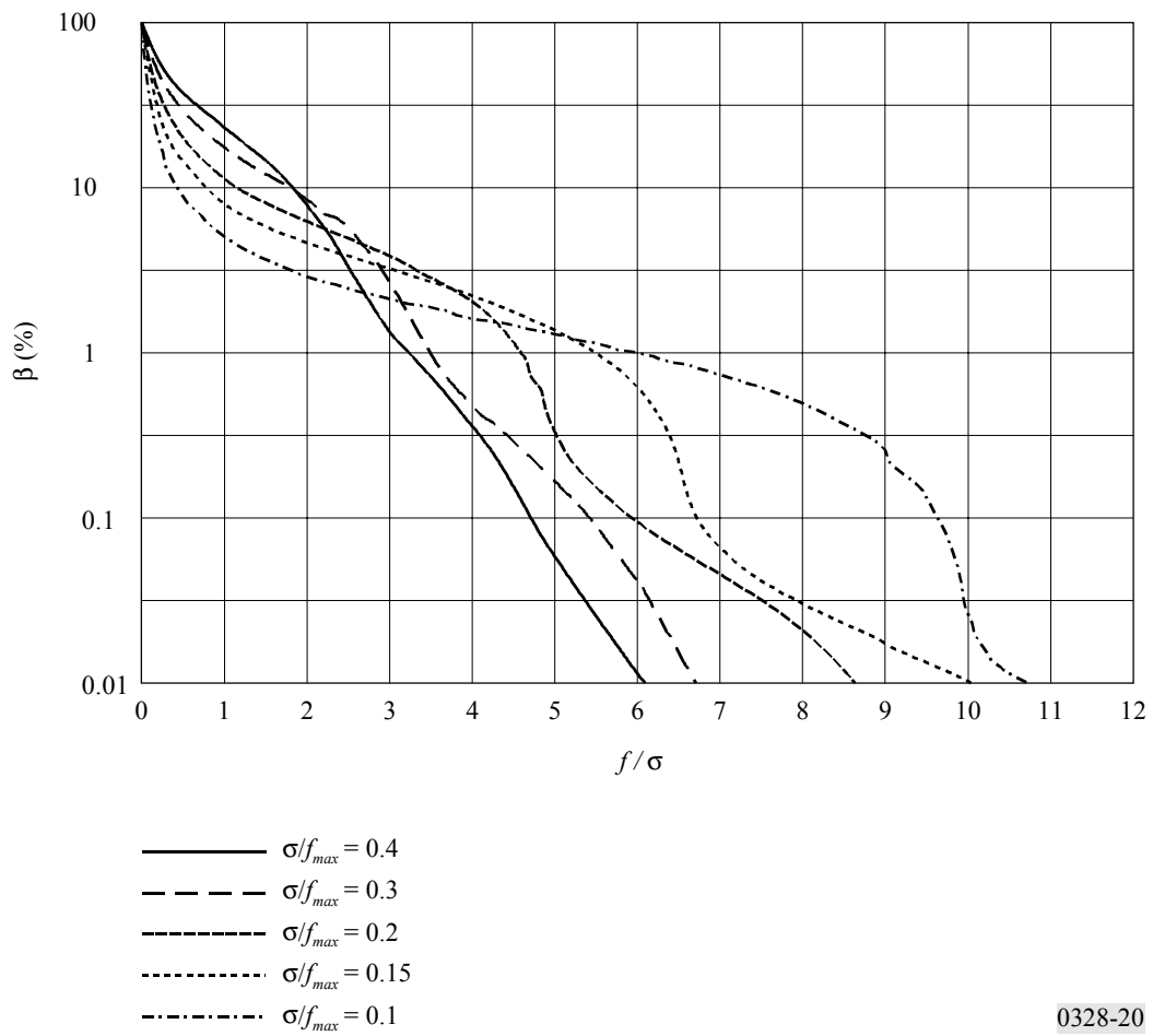
FIGURE 20 Out-of-band power of the spectra for \sigma/f_{max} < 0.5
