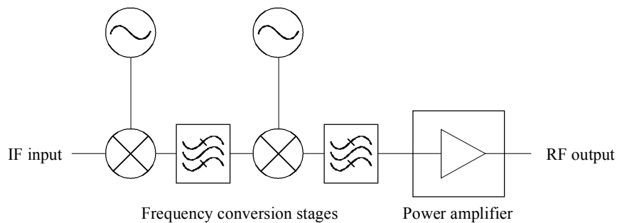
Typical upconversion transmitter architecture
