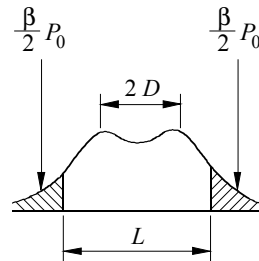
FIGURE 15 Bandwidth calculation from the empirical formula (10)
