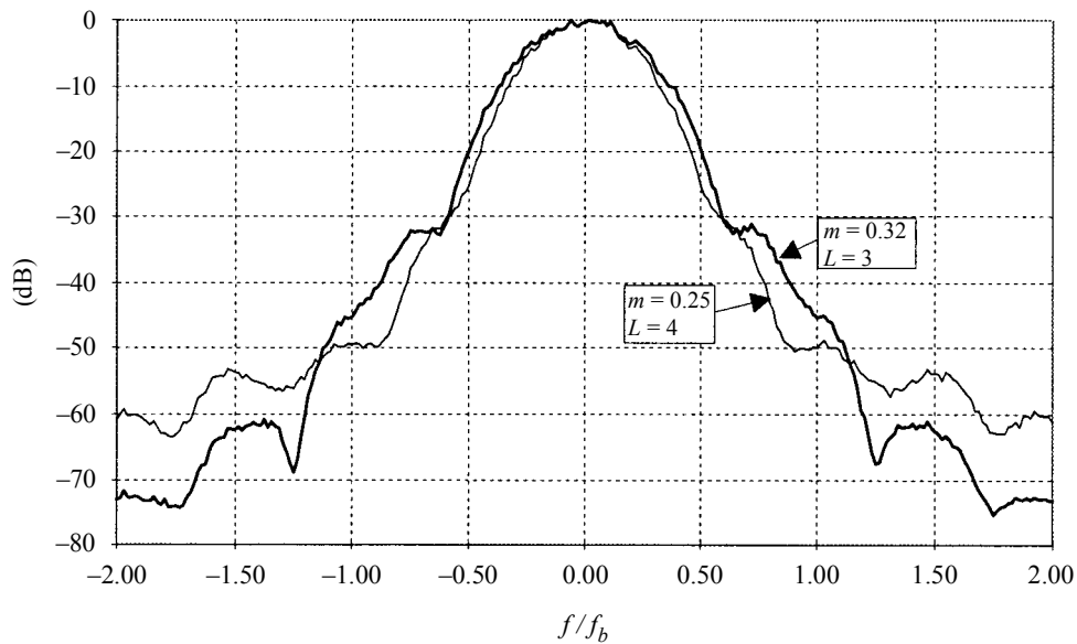
FIGURE 30 Simulated power density spectra for two cases of 2-state CPM ( h = 0.5 )
