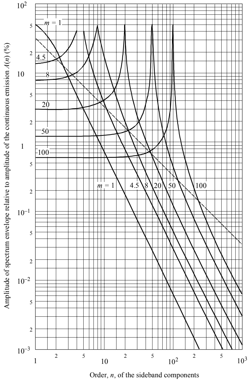
FIGURE 12 Envelopes of RF spectra for a telegraph signal consisting of reversals
