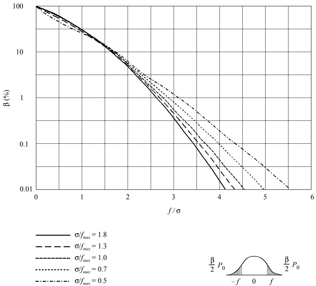
FIGURE 19 Out-of-band power of the spectra for \sigma/f_{max} \geq 0.5
