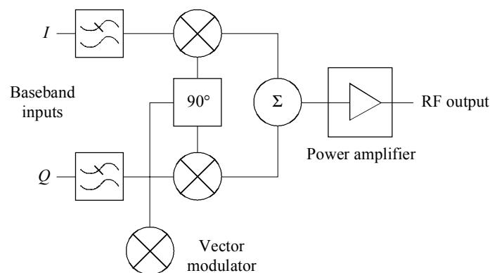
Vector modulator transmitter architecture
