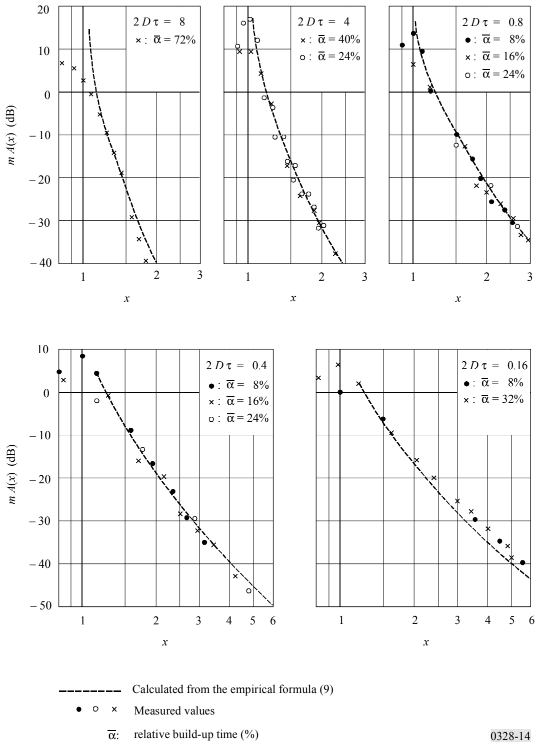
FIGURE 14 Spectra of F1B emissions
